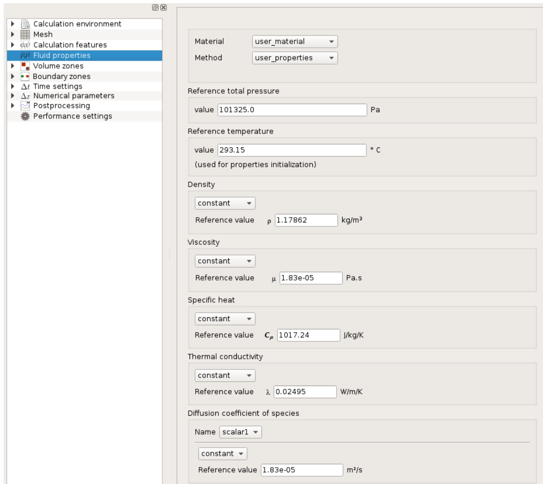
Figure 30: Physical properties - Fluid properties
