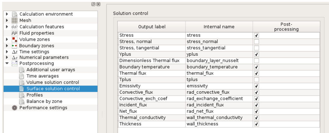
Figure 47: Calculation control - Radiative transfers post-processing output
