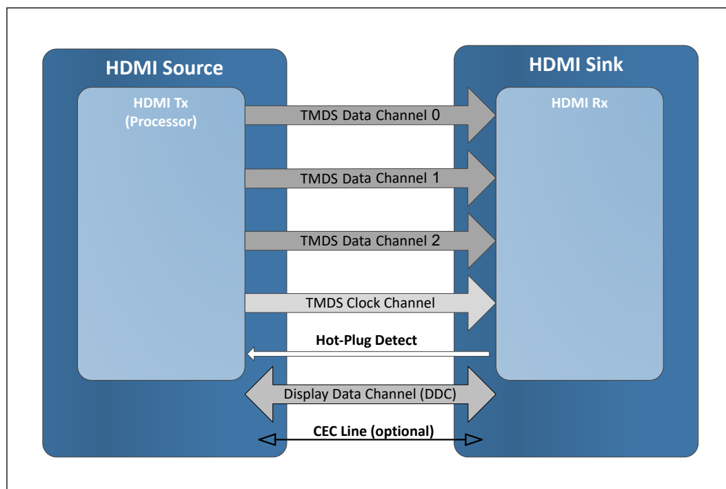
Figure 25. HDMI* Overview
