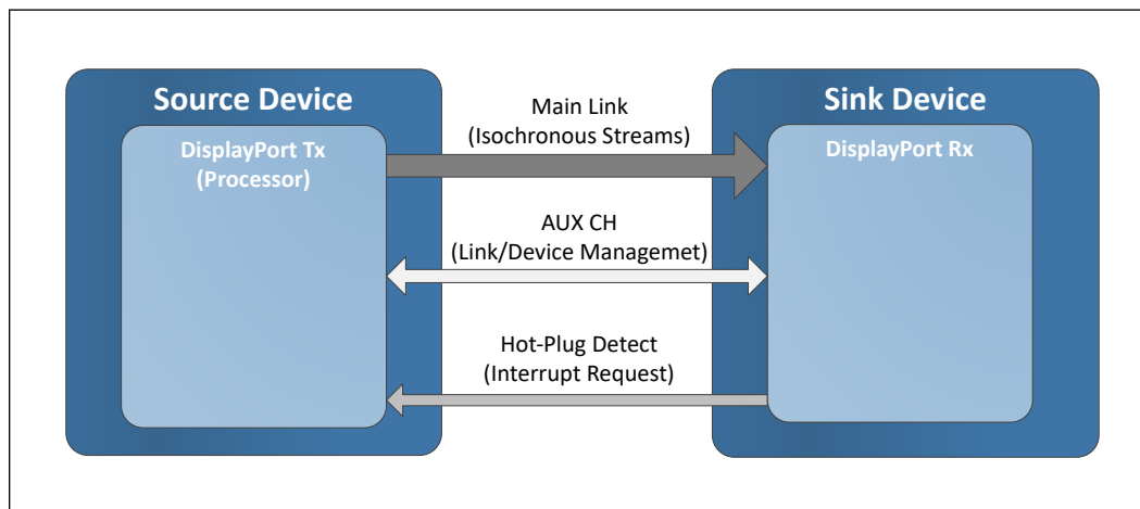
Figure 24. DisplayPort* Overview
