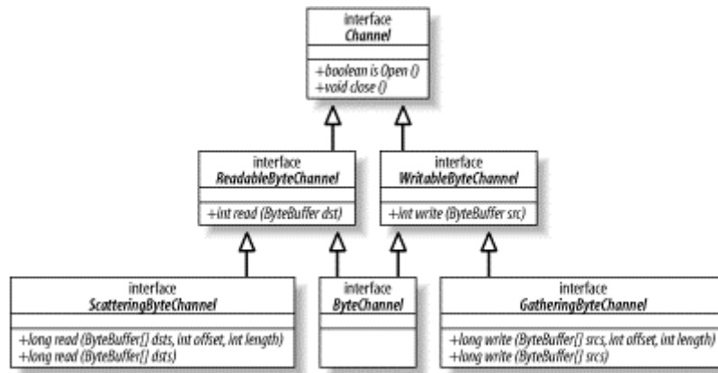
Figure 3-4. Scatter/gather interfaces
