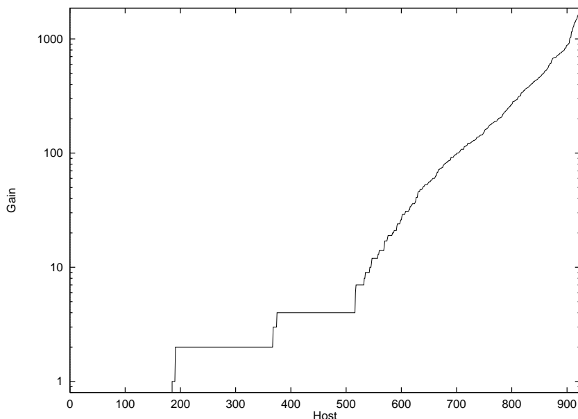
Figure 3: Distribution of gains seen using the broadcast address for Lucent's intranet. The network that generated a gain 43,509 and is excluded from this graph.
