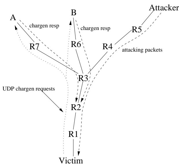
Figure 2: Example of traceback step. Packets are sent to A and B, spoofed from R2, in order to initiate packet flows towards the victim. This causes increases congestion along the R3-R2 link, which, if sufficient, will induce packet loss.
