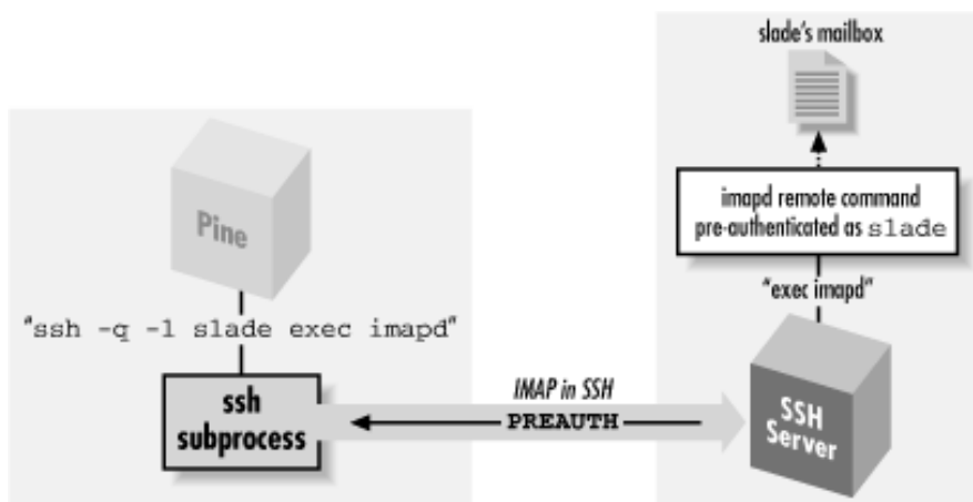
Figure 11.10. Pine/IMAP over SSH, preauthenticated
