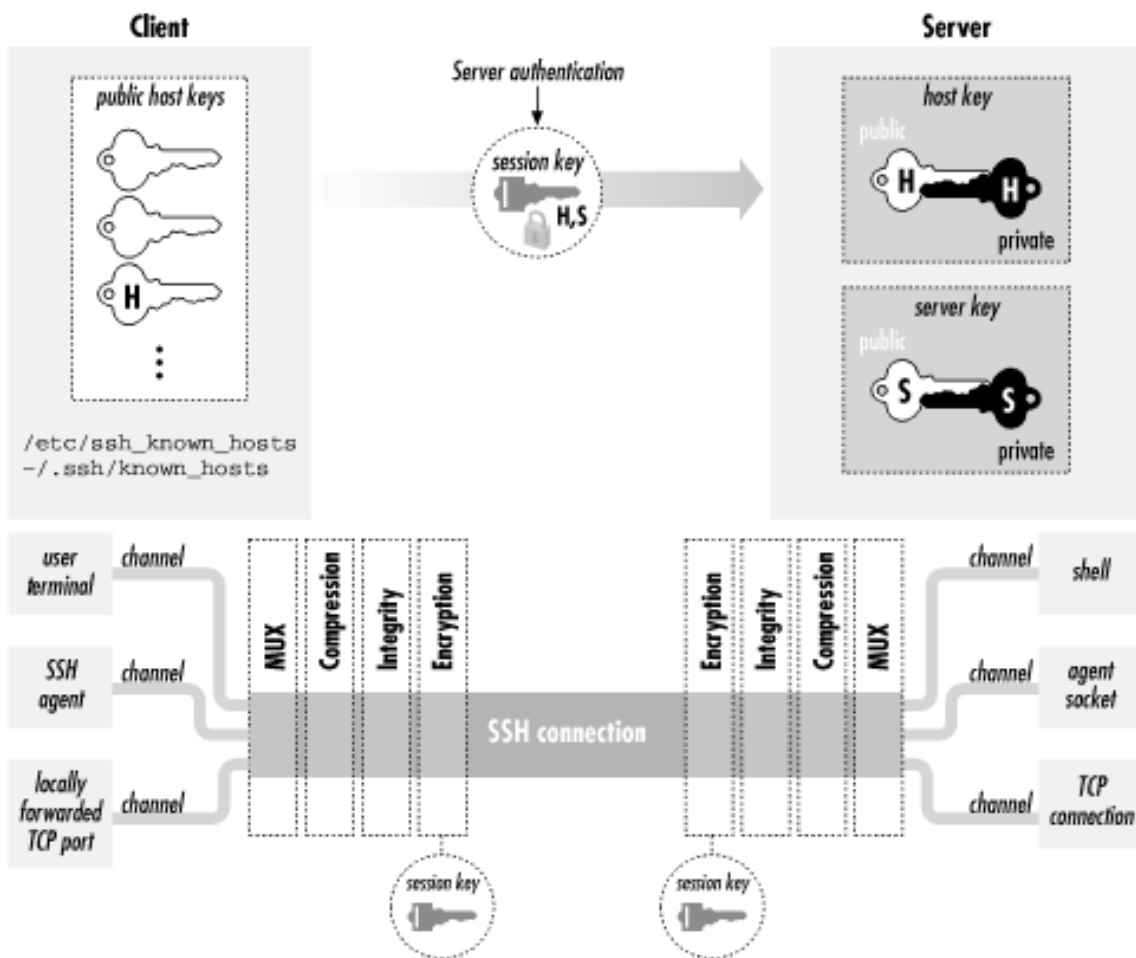
Figure 3.2. SSH-1 architecture
