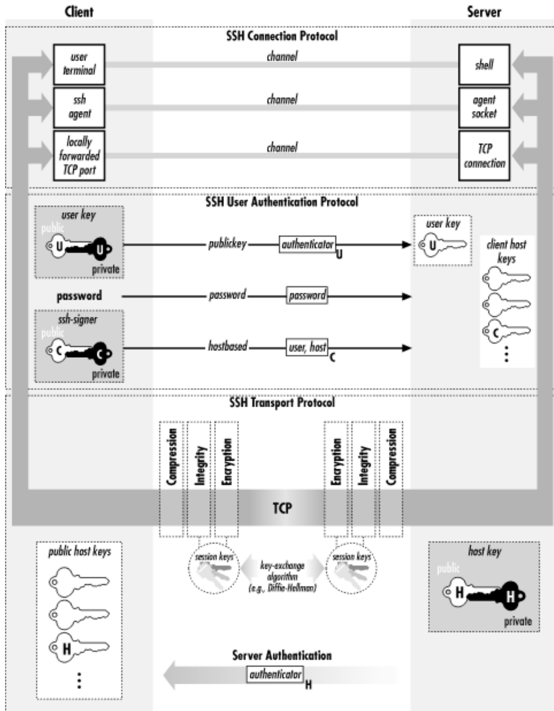
Figure 3.4. SSH-2 architecture
